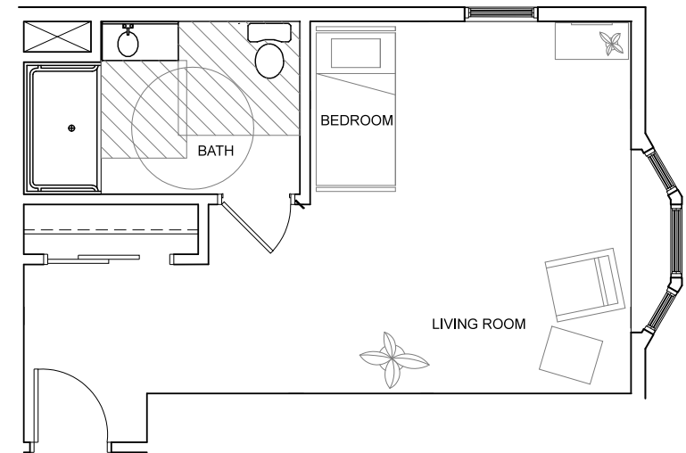
Barrier-free Studio 394 Sq. Ft.
